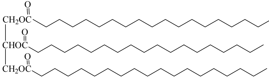
saturated fat (a triglyceride)
